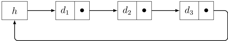
图 3.5: 循环链表 (Circular Linked List)
