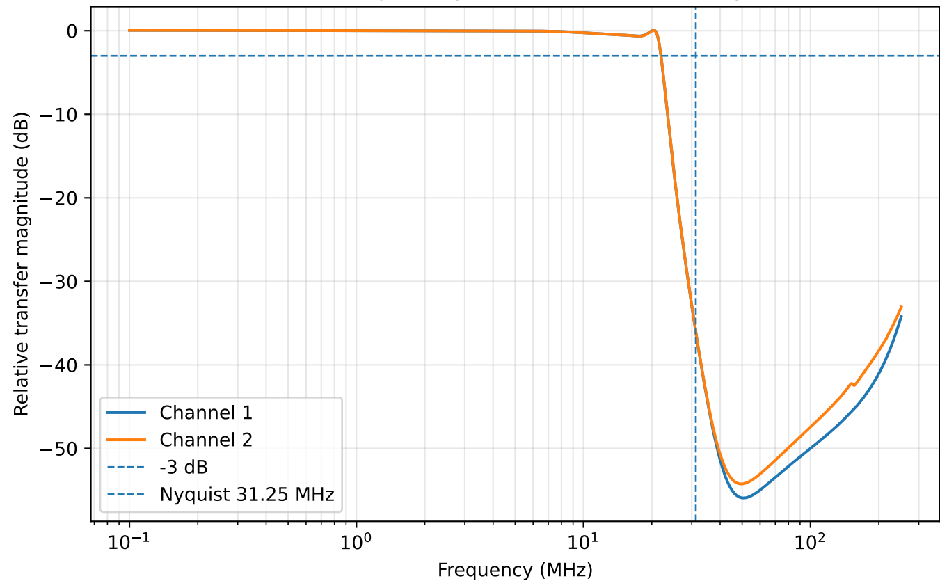
DUAL AAF — post-layout measured-TMUX response
