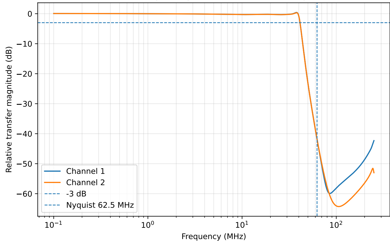
FAST AAF — post-layout measured-TMUX response
