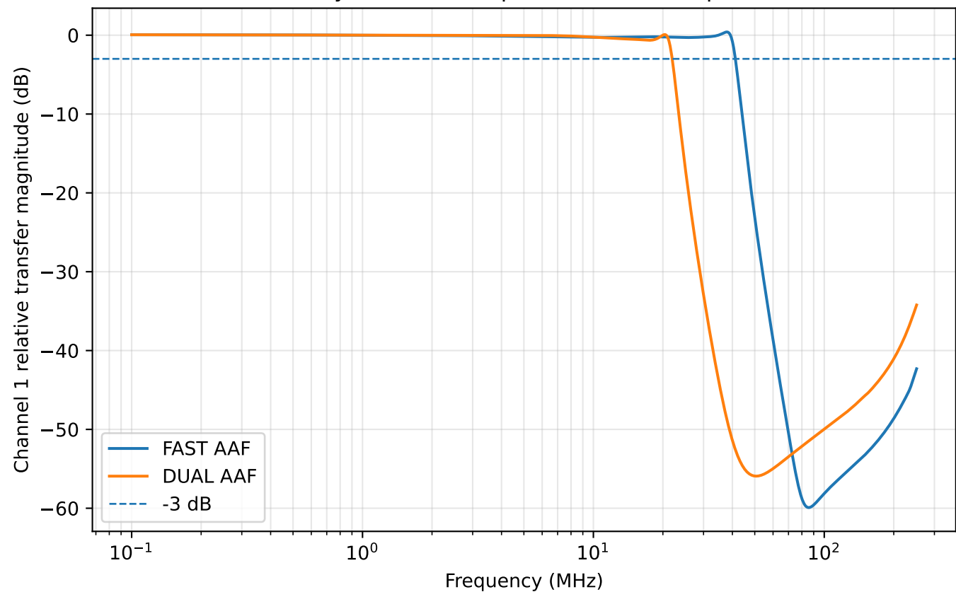
Post-layout oscilloscope AFE mode comparison
