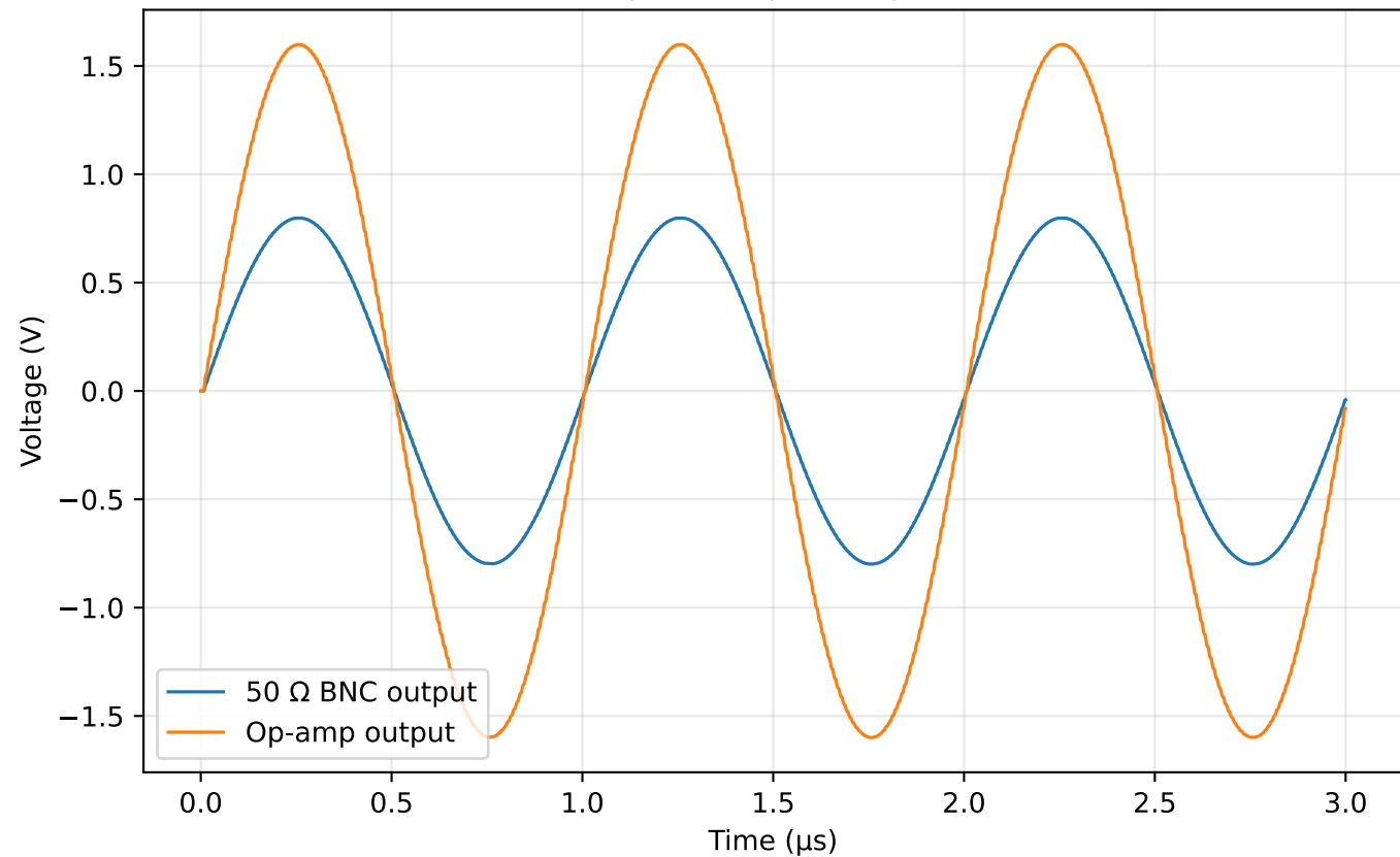
AWG accepted output-stage transient
