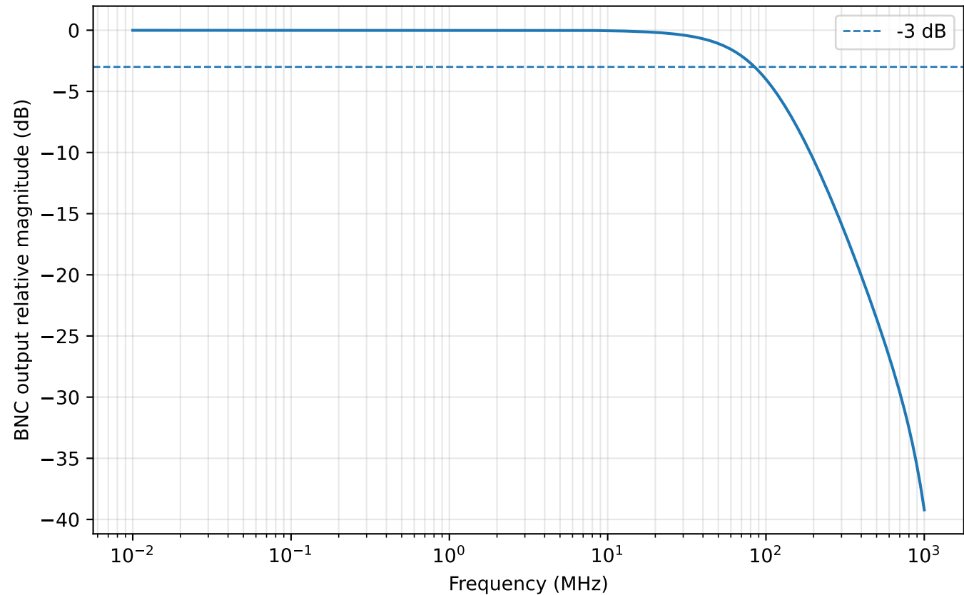
AWG post-layout signal-path AC response
