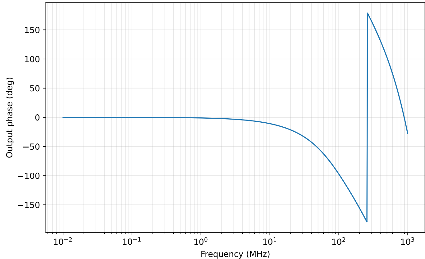
AWG post-layout output phase
