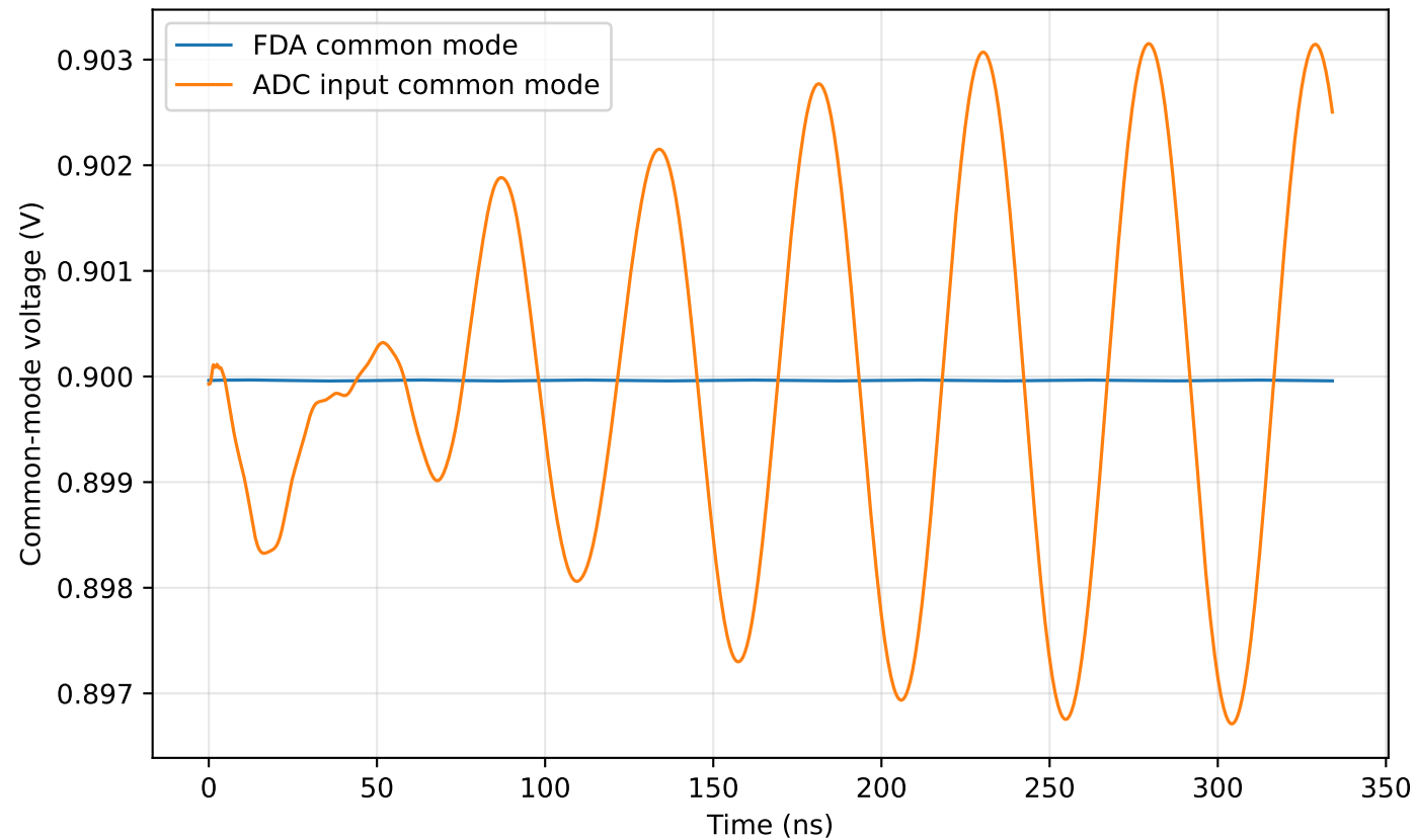
HIGH DUAL 20MHz — common mode
