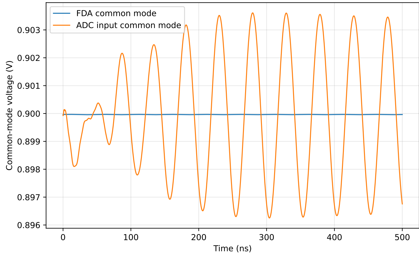
LOW DUAL 20MHz — common mode
