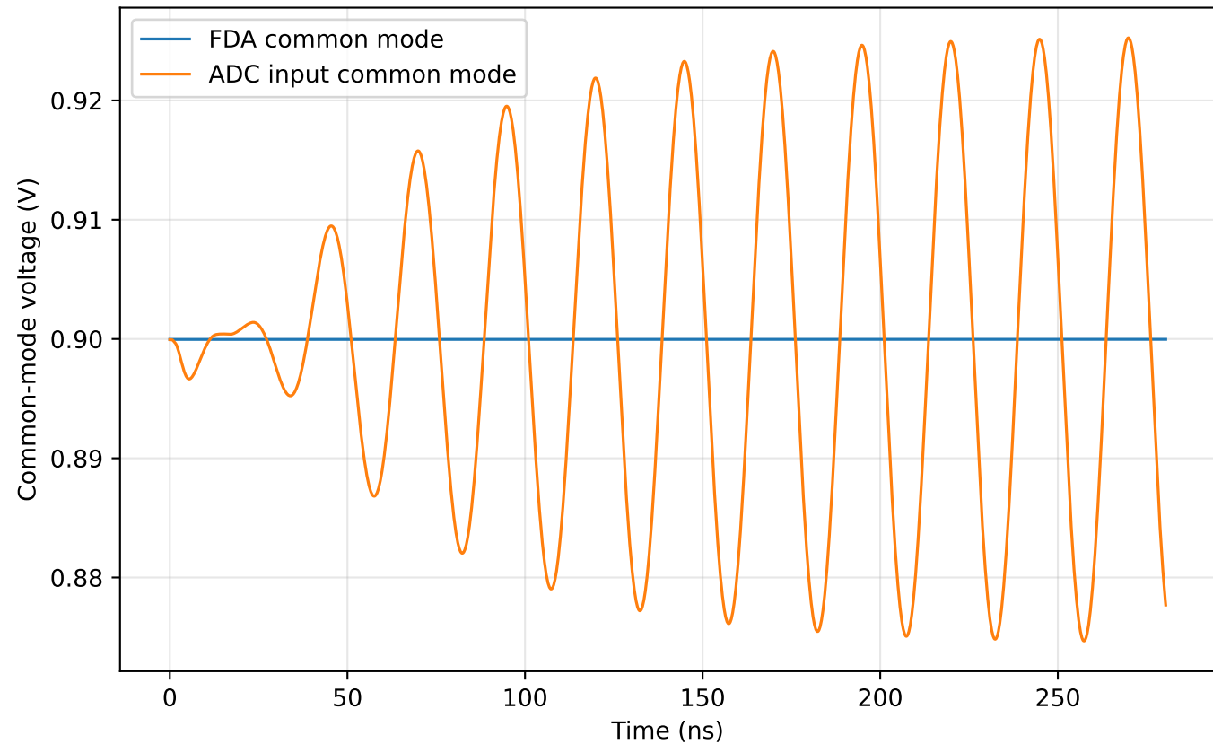
LOW FAST 40MHz — common mode
