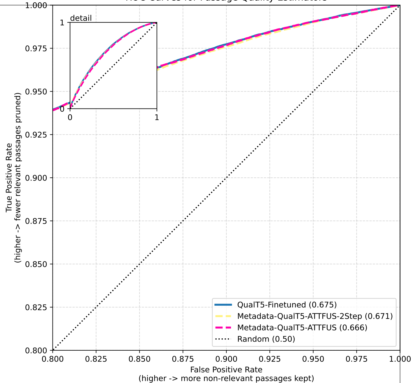
ROC Curves for Passage Quality Estimators
