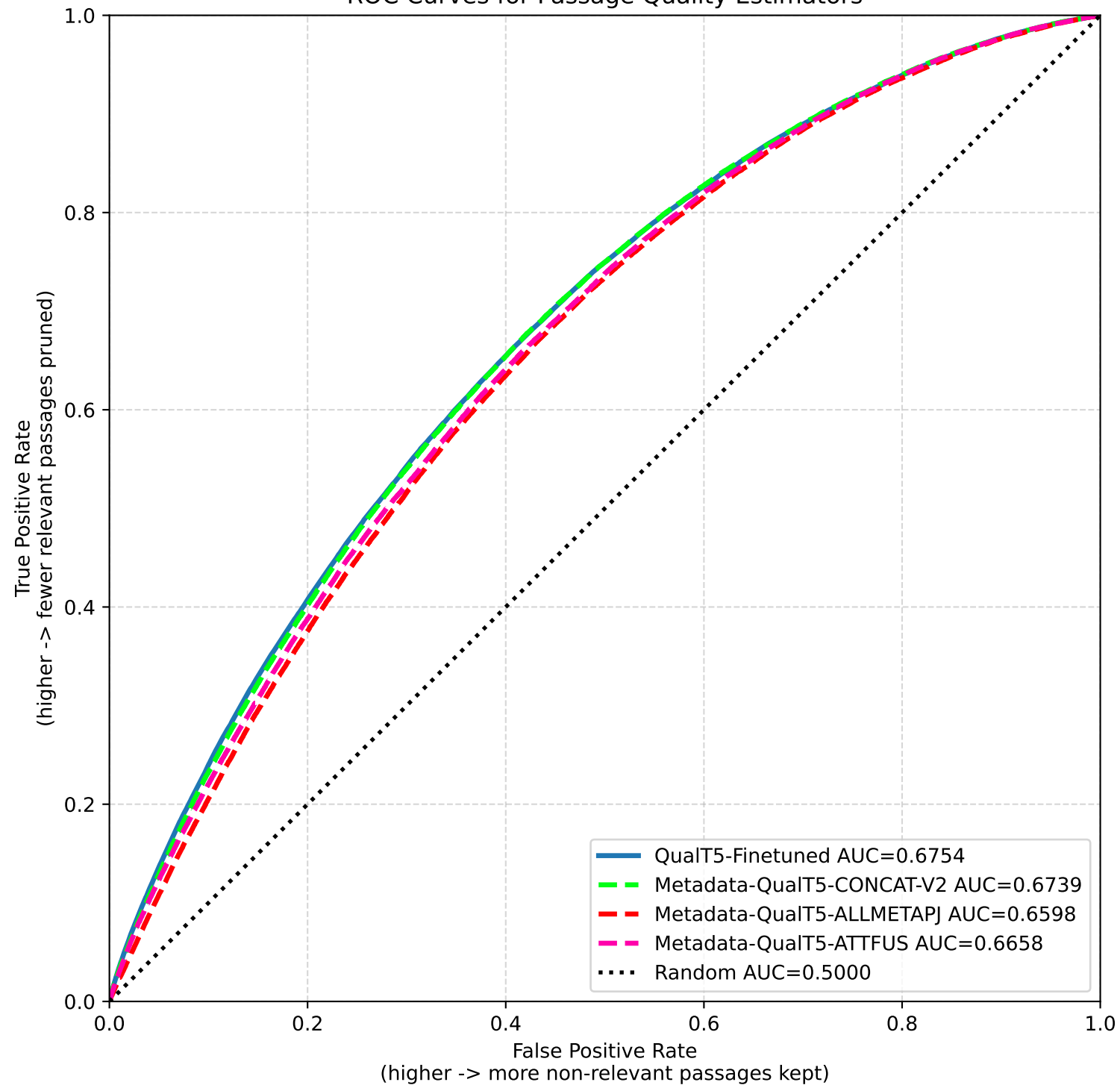
ROC Curves for Passage Quality Estimators
