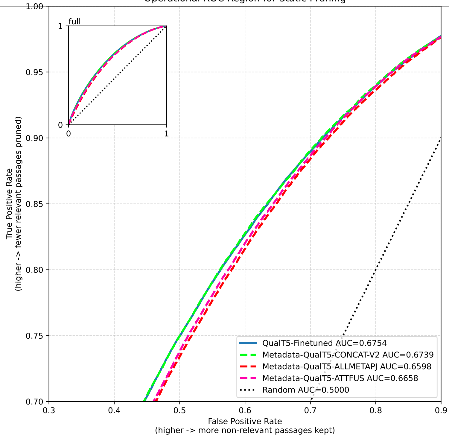
Operational ROC Region for Static Pruning
