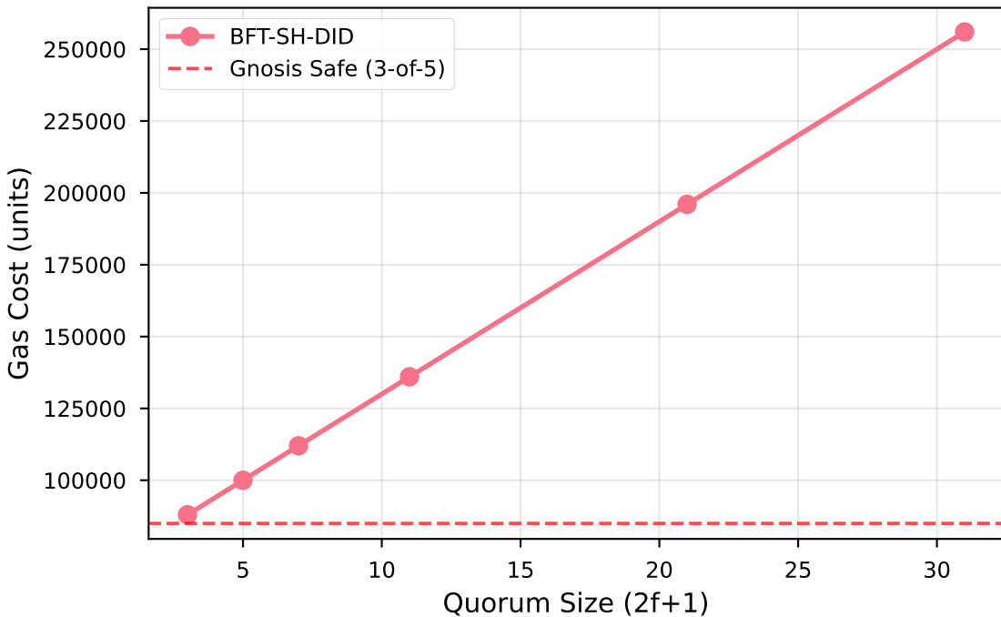
BFT-SH-DID: Recovery Gas Cost vs. Quorum Size
