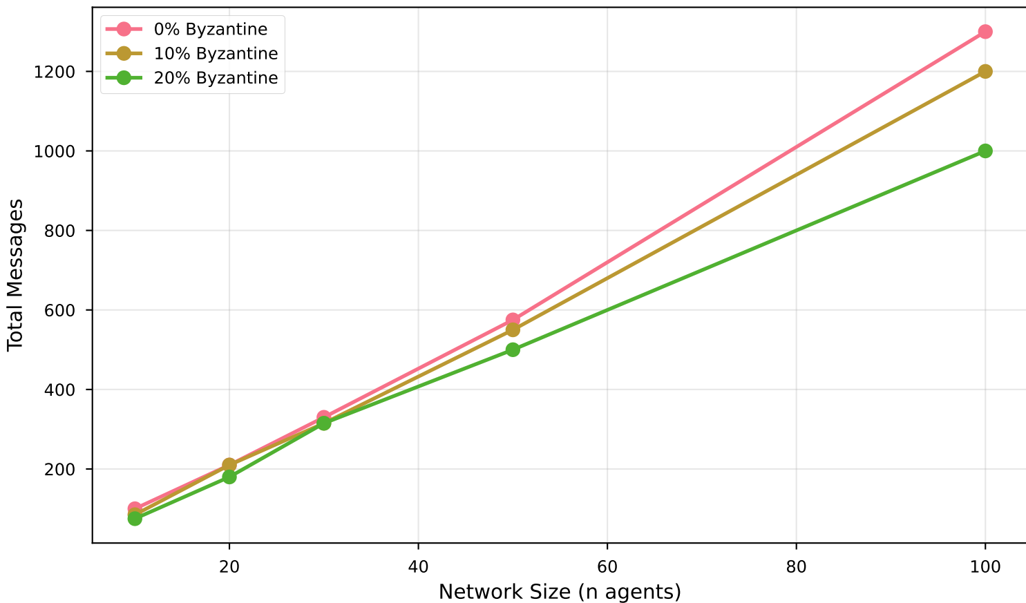
BFT-MV-DID: Communication Overhead
