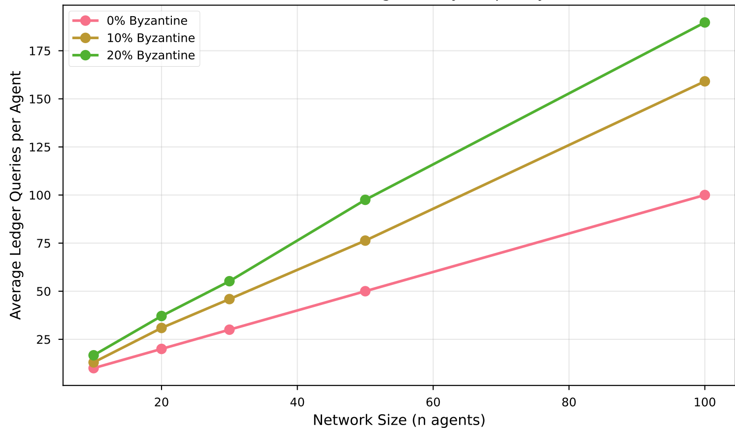
BFT-MV-DID: Ledger Query Frequency
