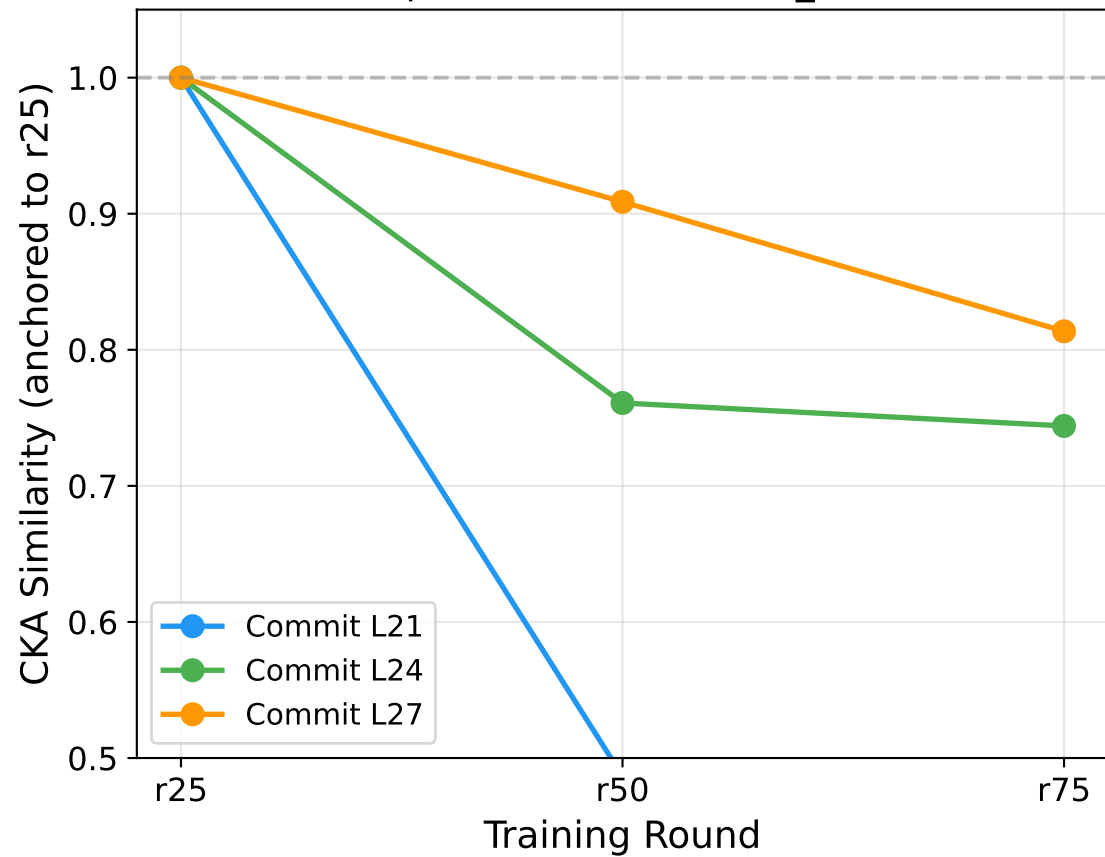
Representation Drift (ts_full)
