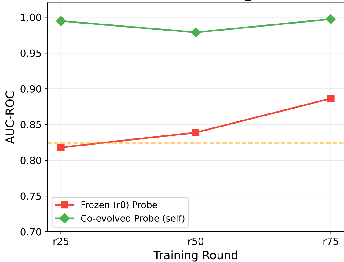
Probe Performance (ts_full)
