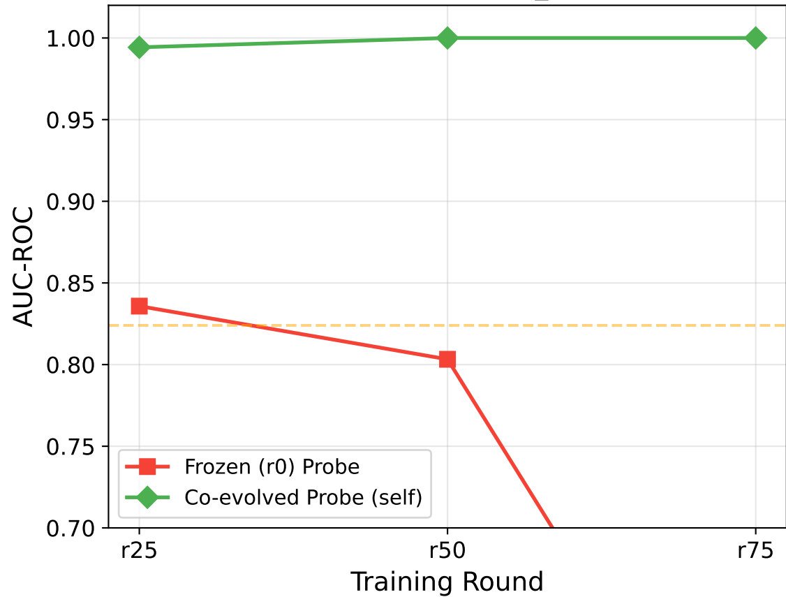
Probe Performance (ts_nogate)
