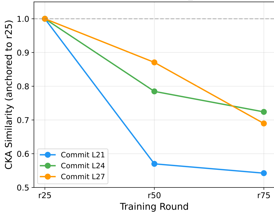
Representation Drift (ts_nogate)
