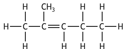
2-methylpent-2-ene
