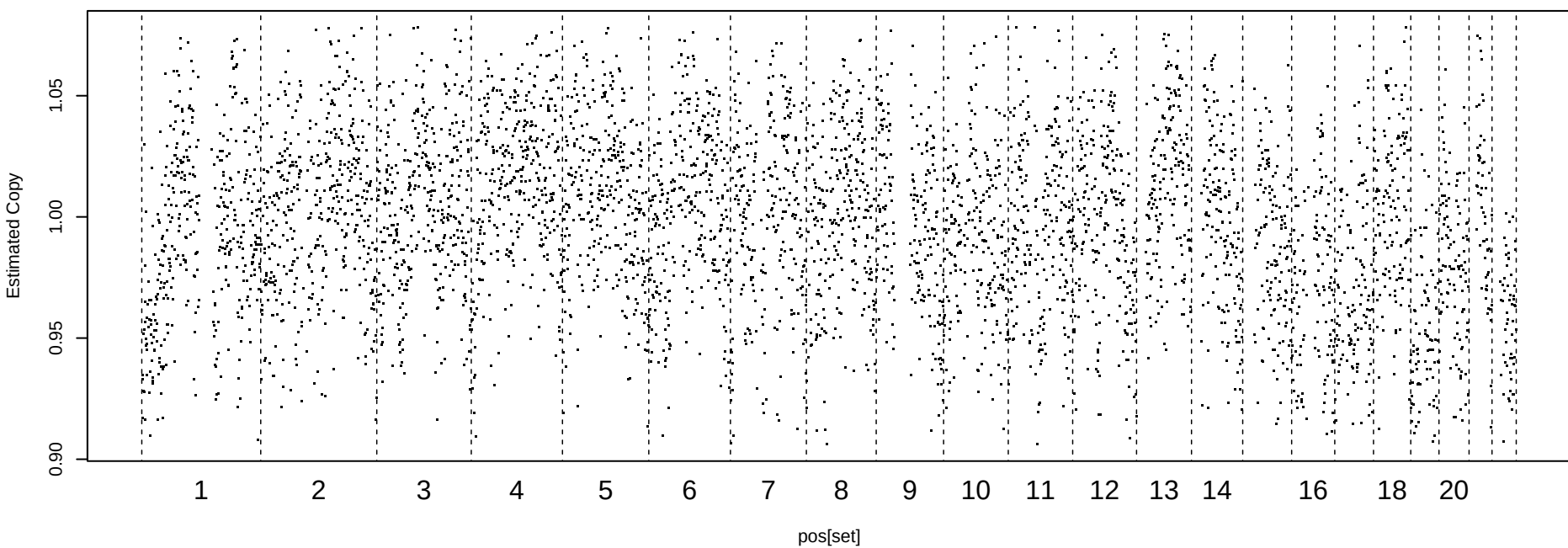
Uncorrected Readcount, MAD = 0.0379
