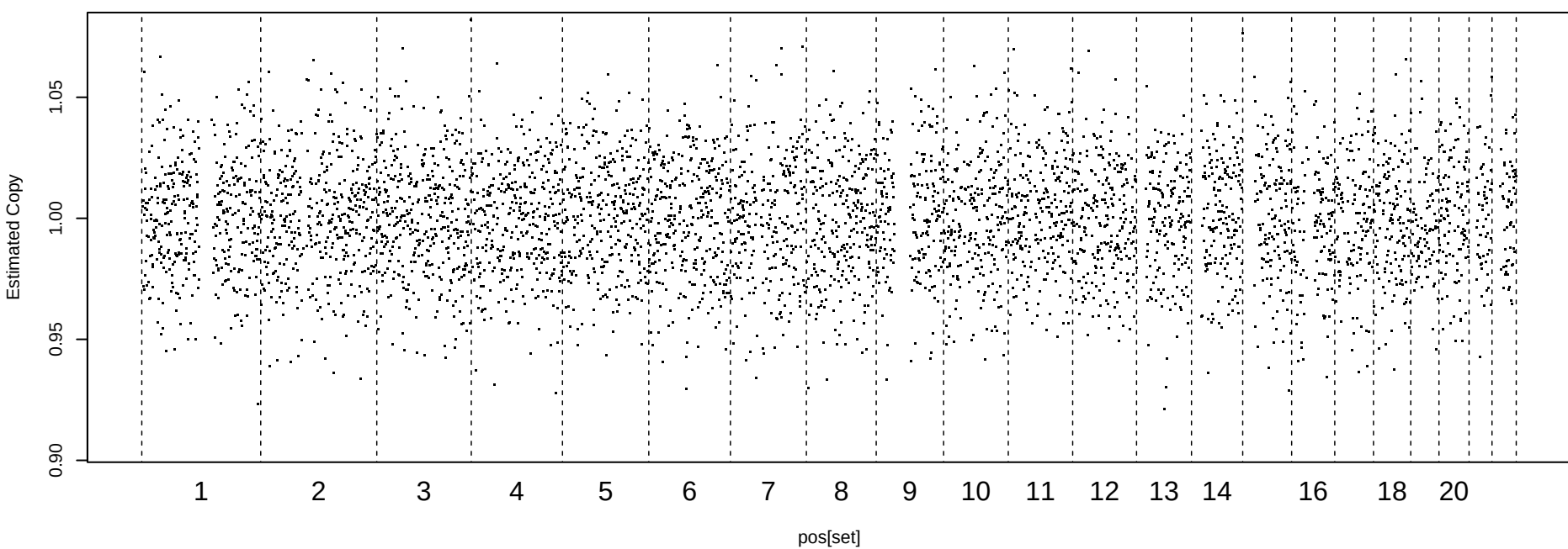
Mappability and GC-corrected Readcount, MAD = 0.0236
