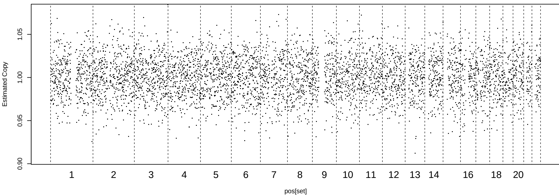
CG-corrected Readcount, MAD = 0.0237
