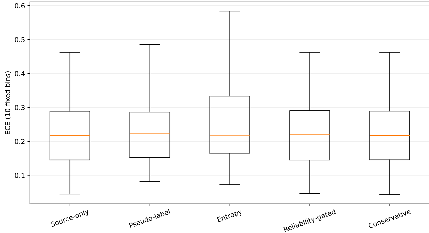
Calibration error across seed-direction evaluations
