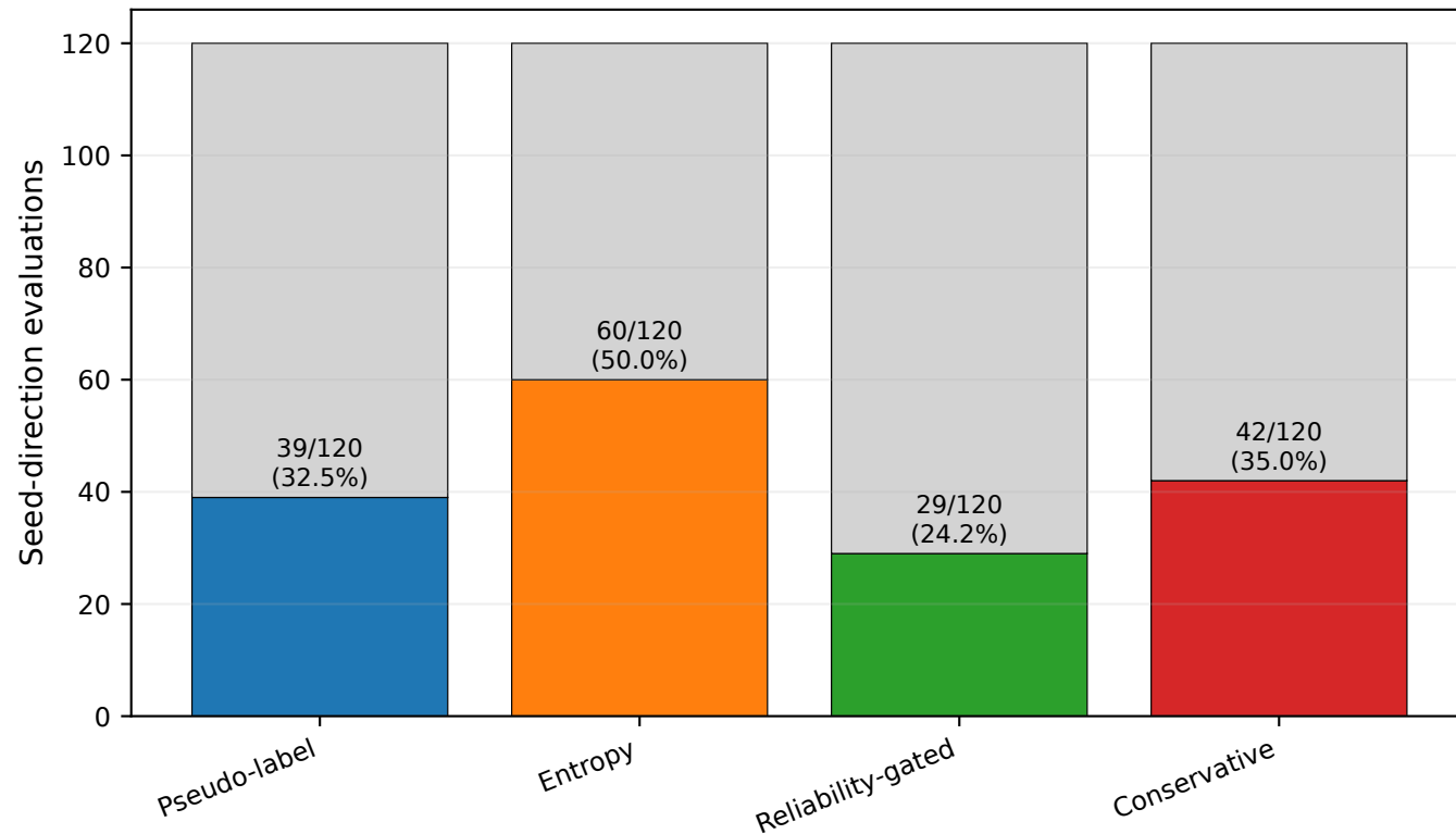
AUROC Negative Adaptation
