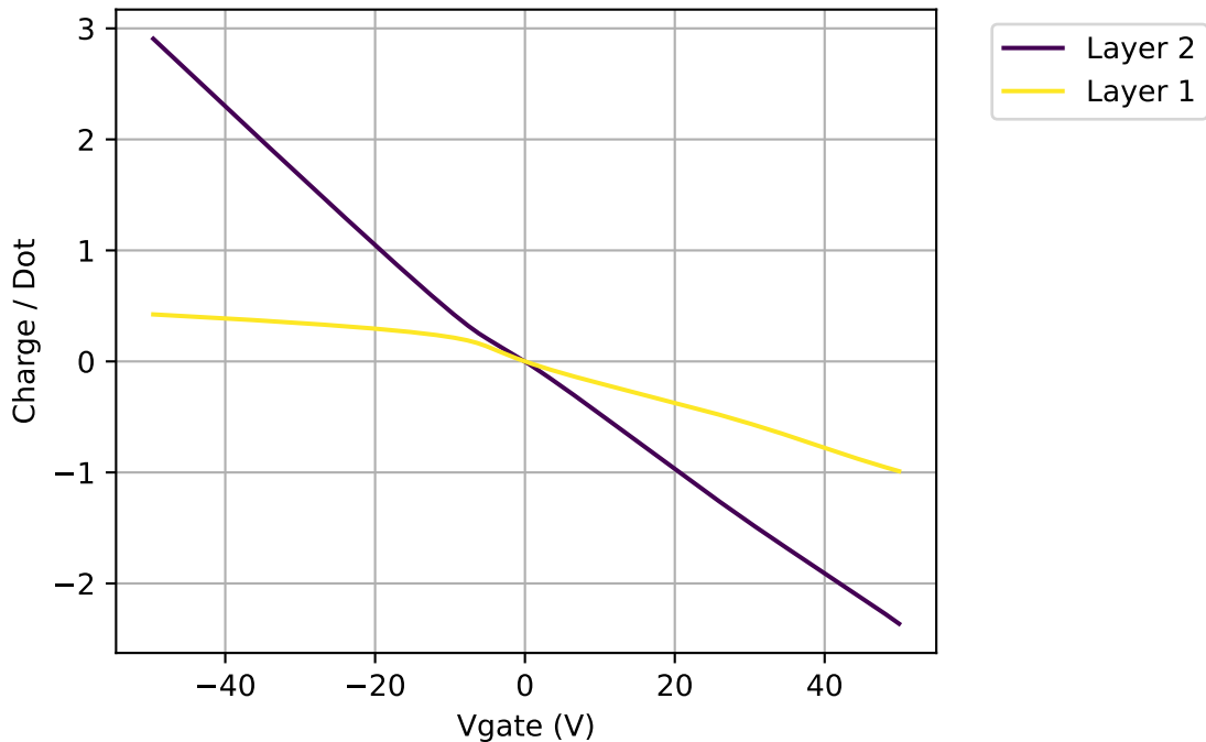
Layer Charge vs Gate Voltage
