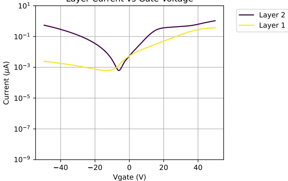
Layer Current vs Gate Voltage
