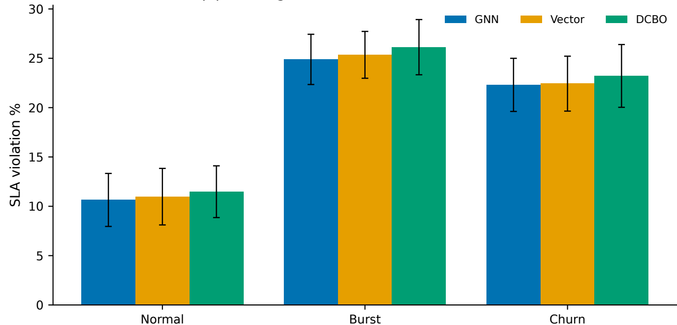
Multipipe tuning lock — SLA at N=100 ( \pm std, 5 trials)
