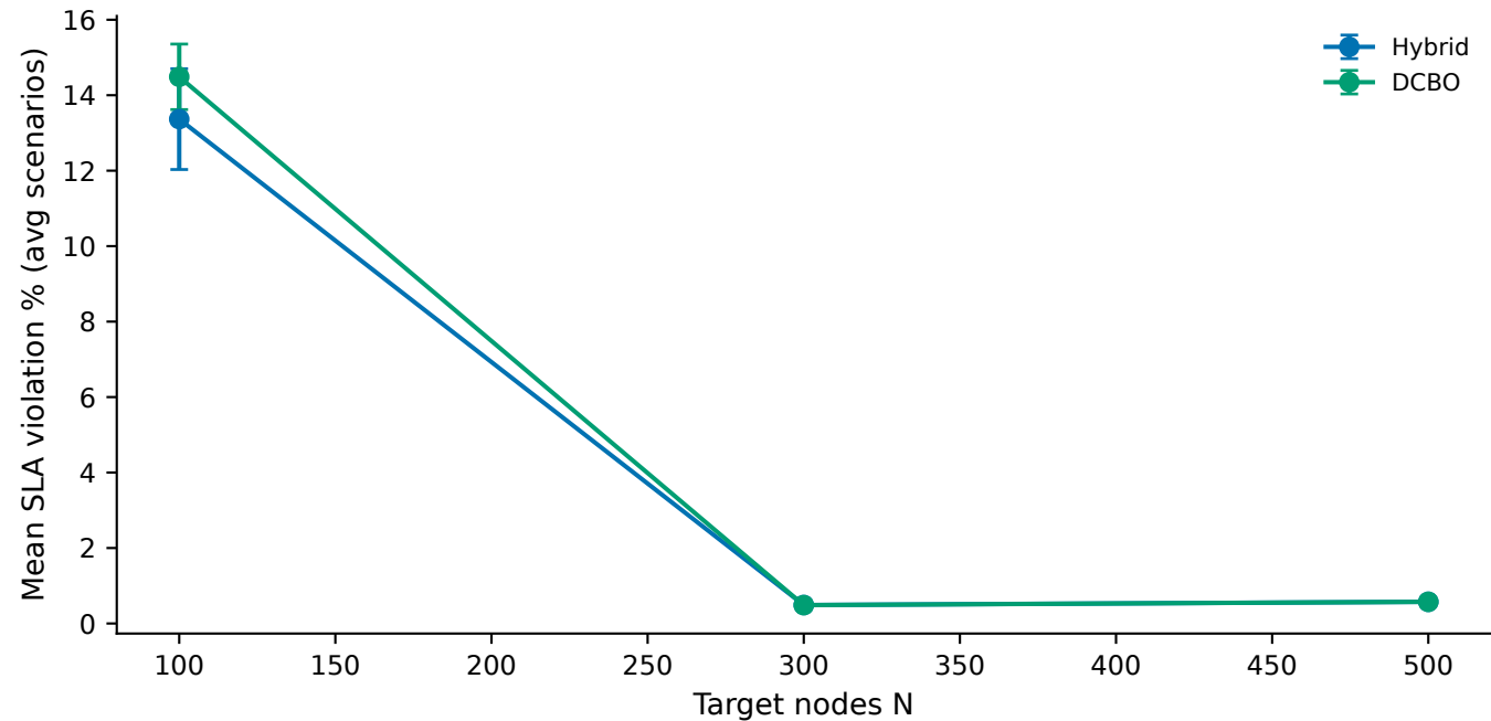
Surveillance — SLA vs scale
