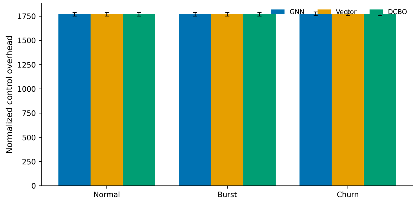
Matched control overhead at N=100 (multipipe champion)
