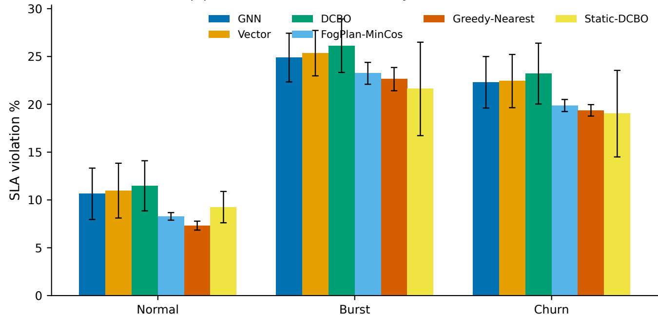
Multipipe N=100 — baselines vs DynaCol-GNN (5 trials)
