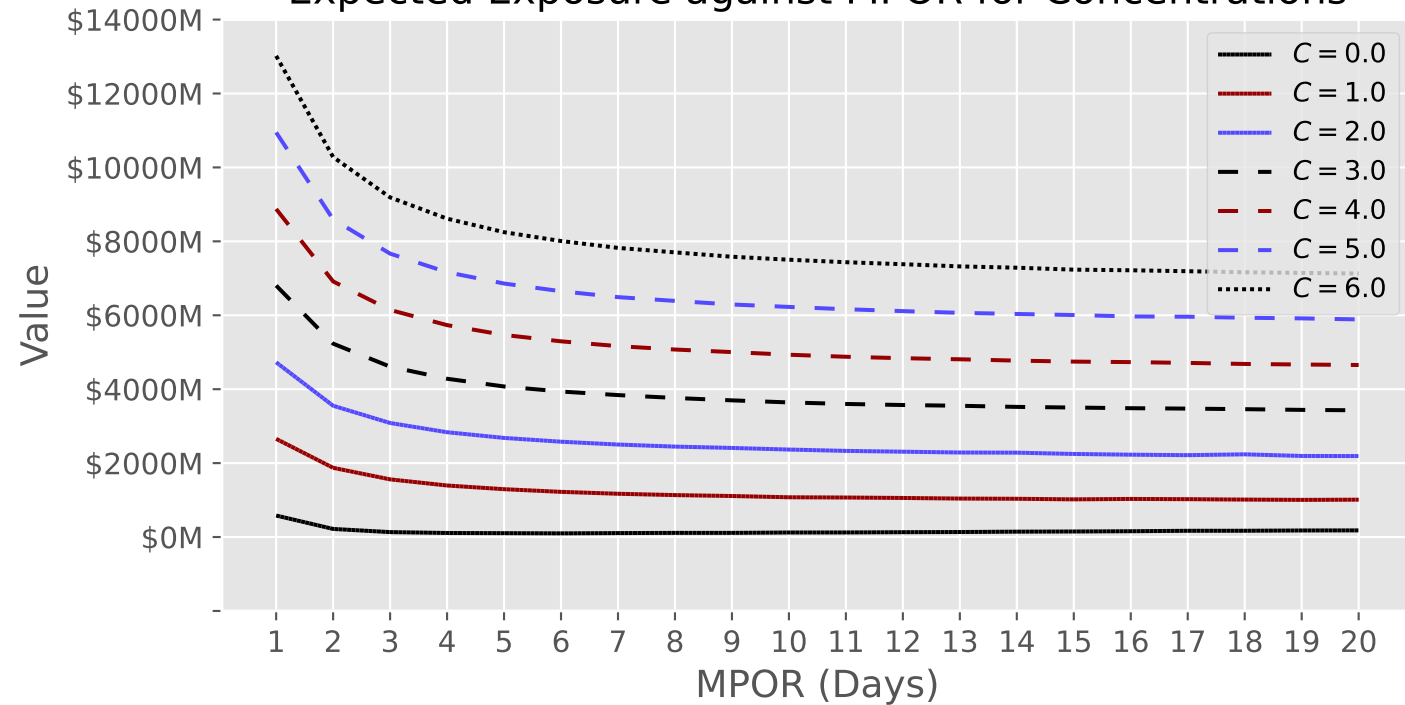
Expected Exposure against MPOR for Concentrations
