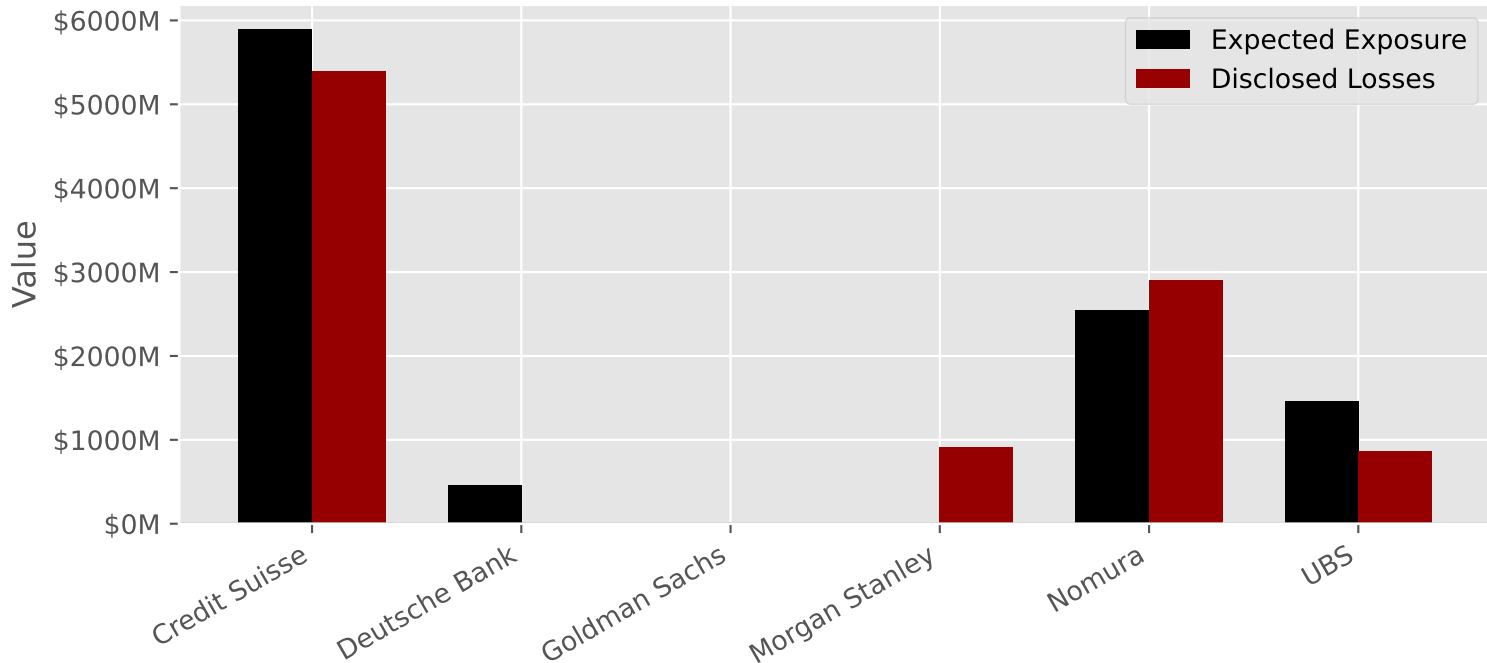
Expected Exposure vs Disclosed Losses by Agent, Alternative Impact Model
