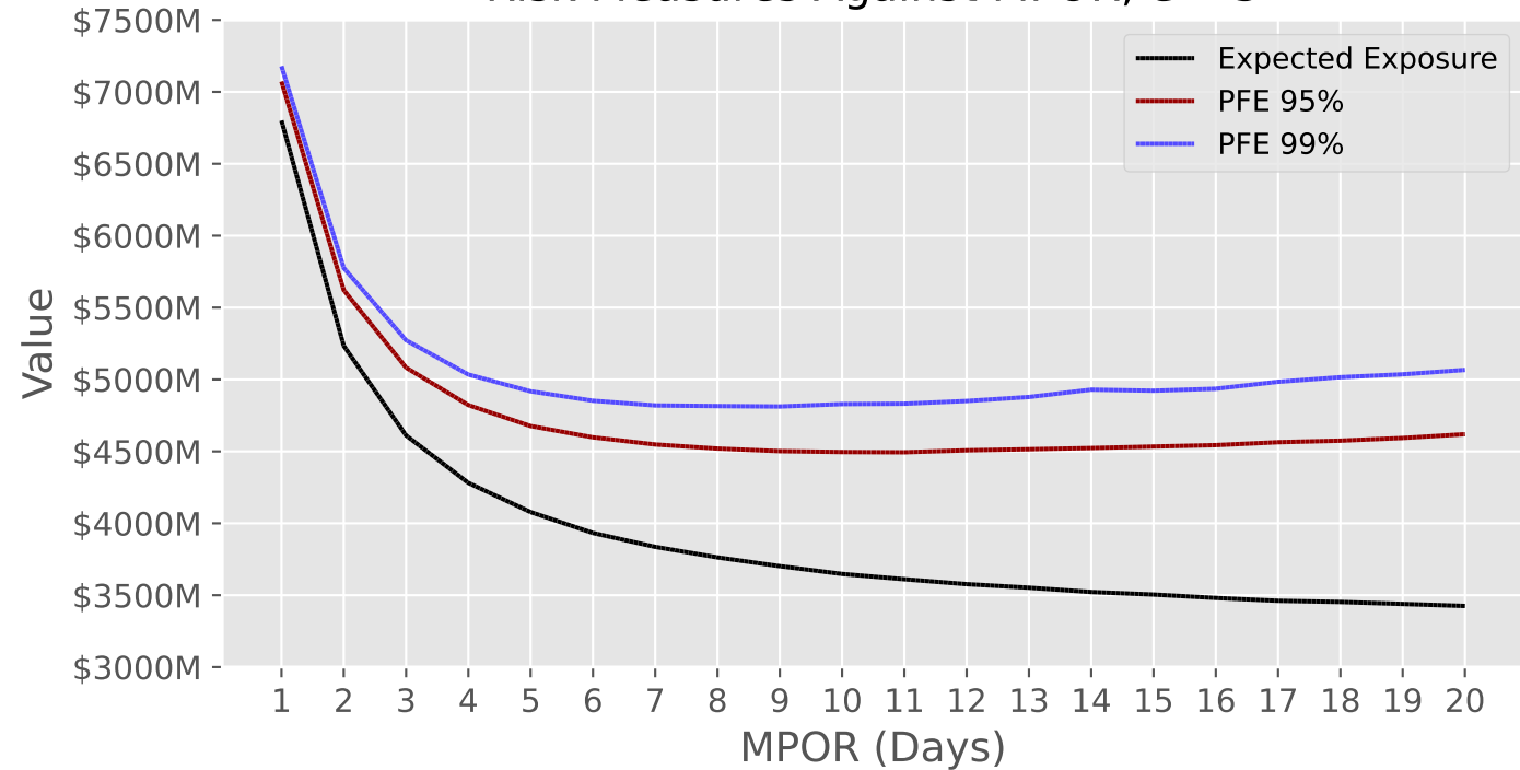
Risk Measures Against MPOR, C = 3
