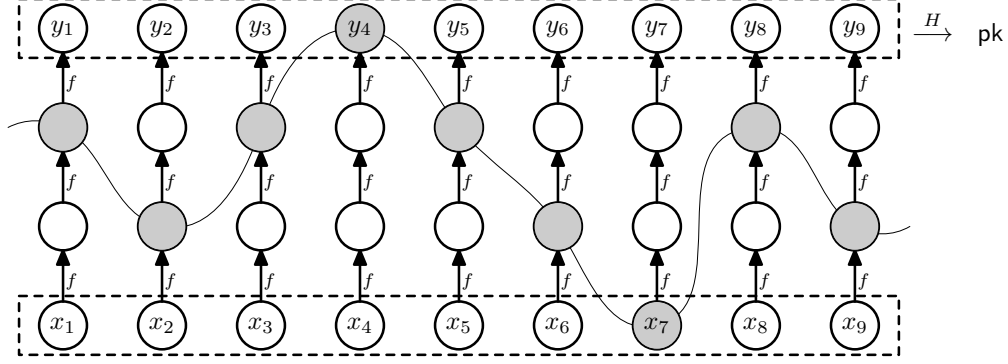
Figure 2: The rectangle of values generated during WOTS key generation with \ell = 9 and d = 4 . The shaded nodes represent a signature on a particular message m where P(m) = (2, 1, 2, 3, 2, 1, 0, 2, 1) .
