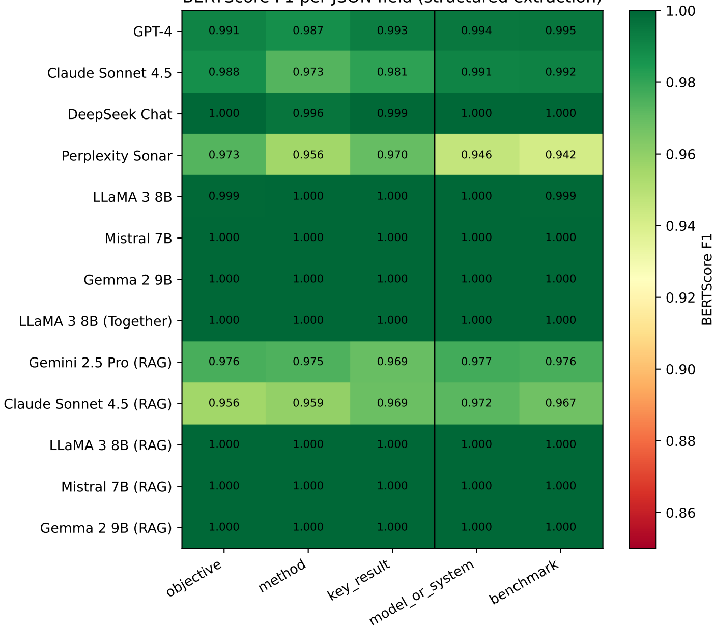
BERTScore F1 per JSON field (structured extraction)
