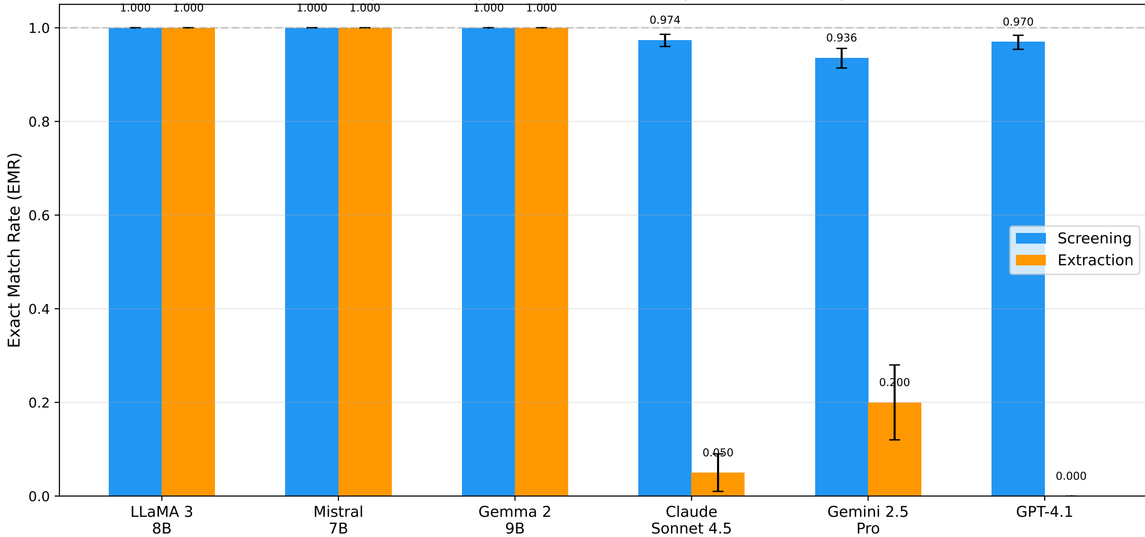
Reproducibility: Exact Match Rate by Model and Stage
