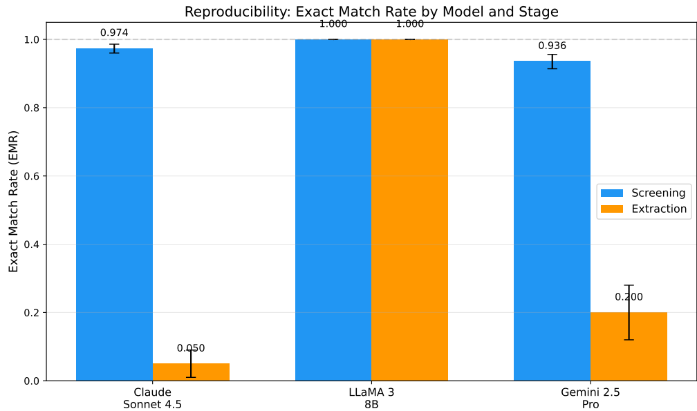
Figure 1: Exact Match Rate (EMR) by model and pipeline stage. Error bars represent 95% bootstrap confidence intervals. The dashed line indicates perfect reproducibility (EMR=1.0).
