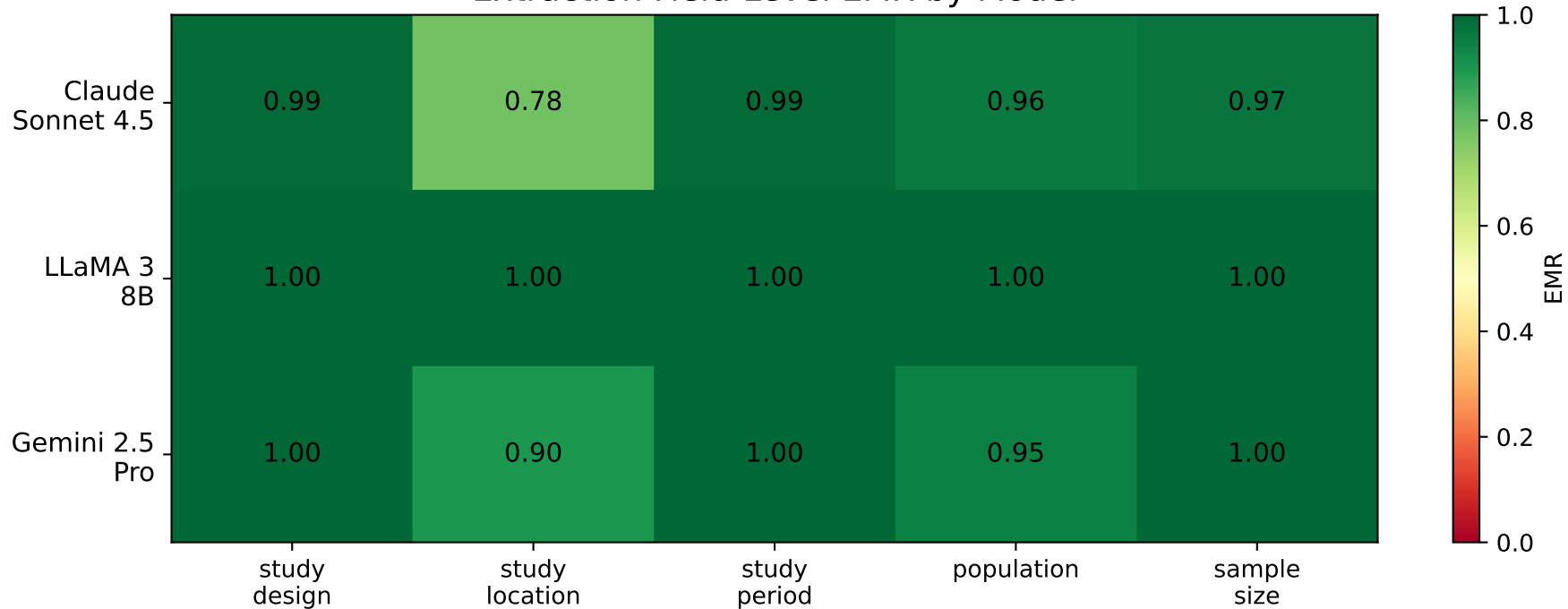
Extraction Field-Level EMR by Model
