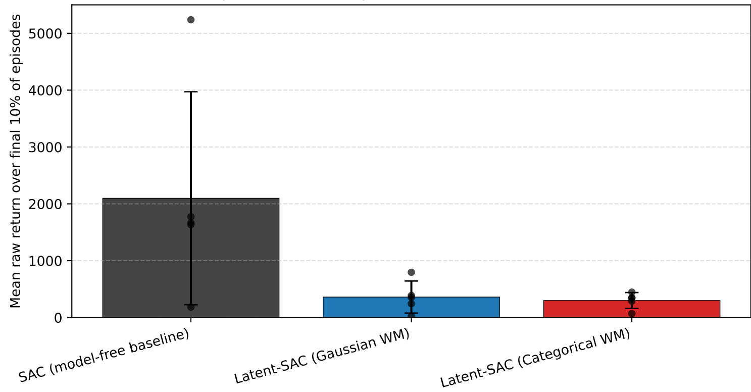
Experiment 3: final performance on HalfCheetah-v5
