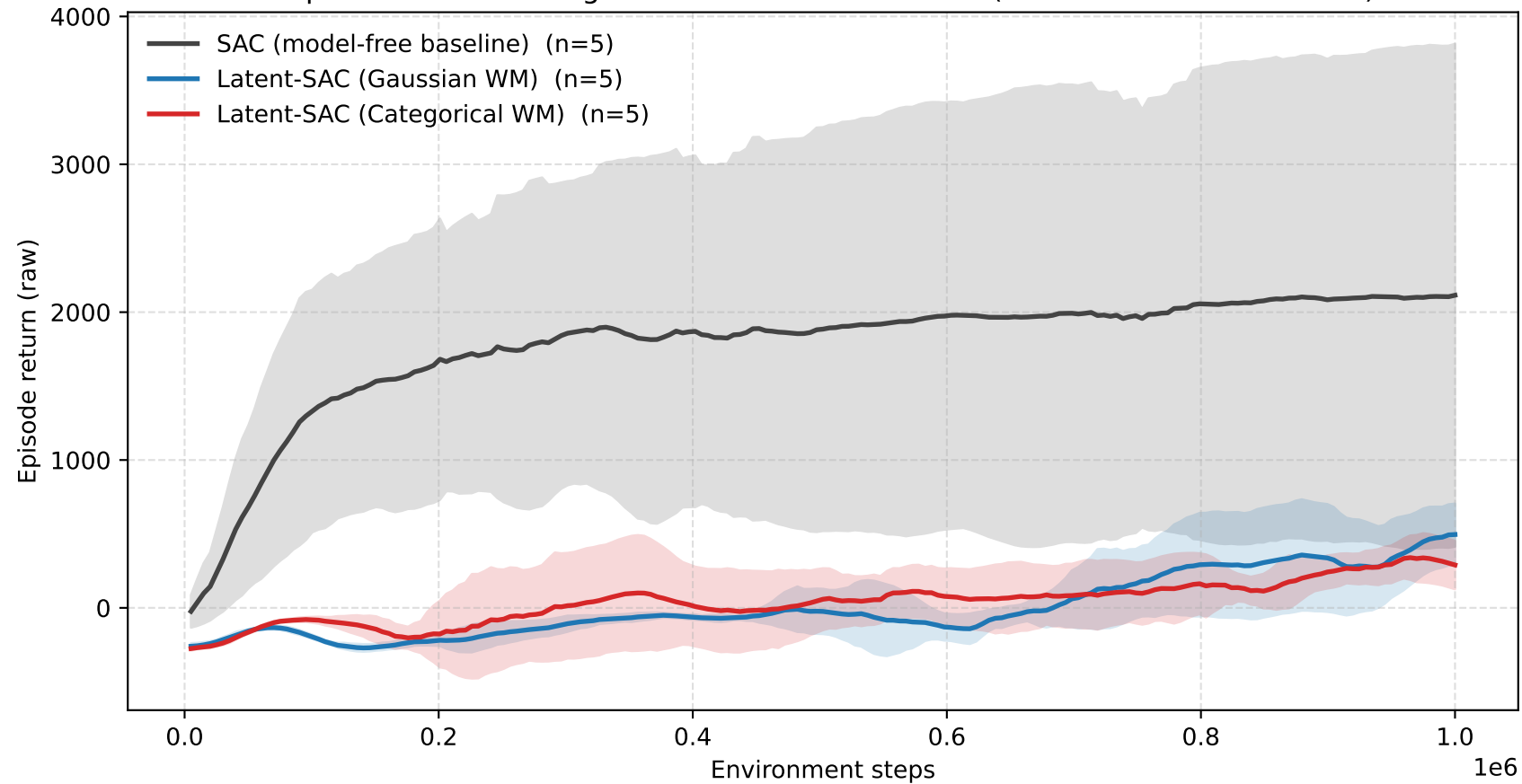
Experiment 3: learning curves on HalfCheetah-v5 (mean \pm 1 std over seeds)
