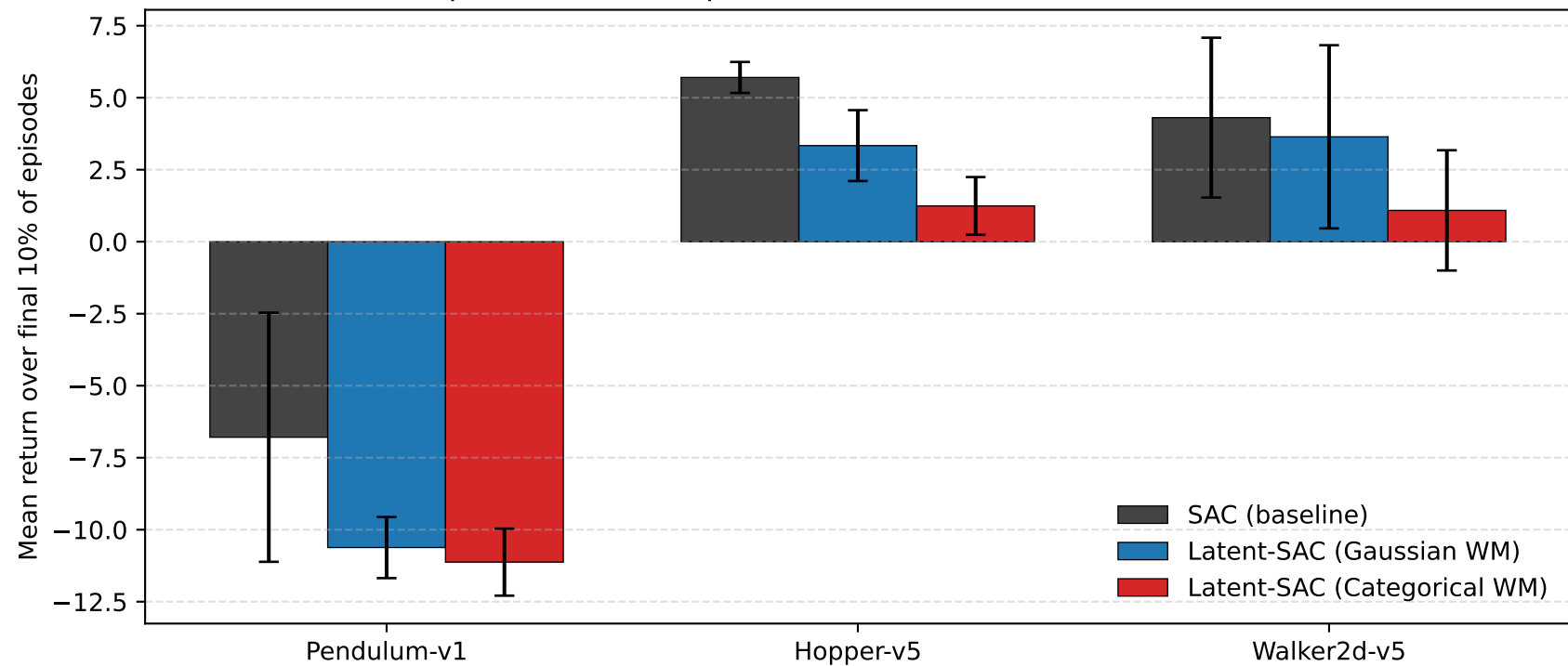
Experiment 1: final performance (mean \pm std over 3 seeds)
