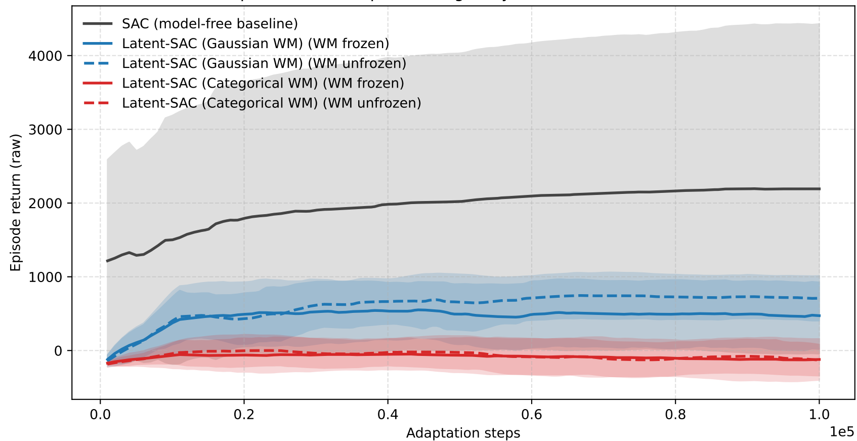
Experiment 4: adaptation to gravity \times 1.5 on HalfCheetah-v5
