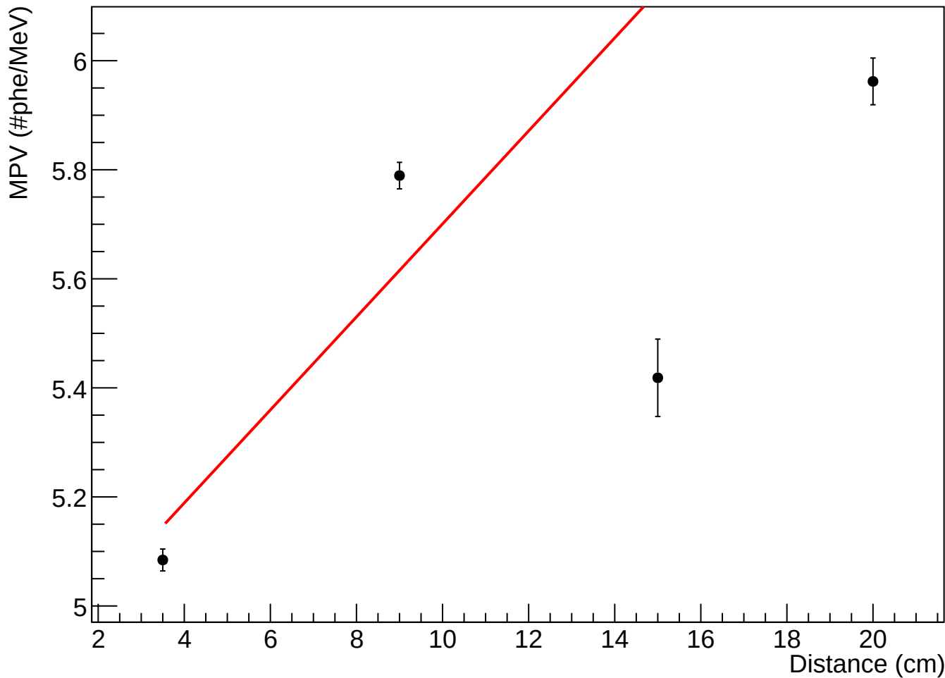
MPV vs Distance from SiPM (using amp)
