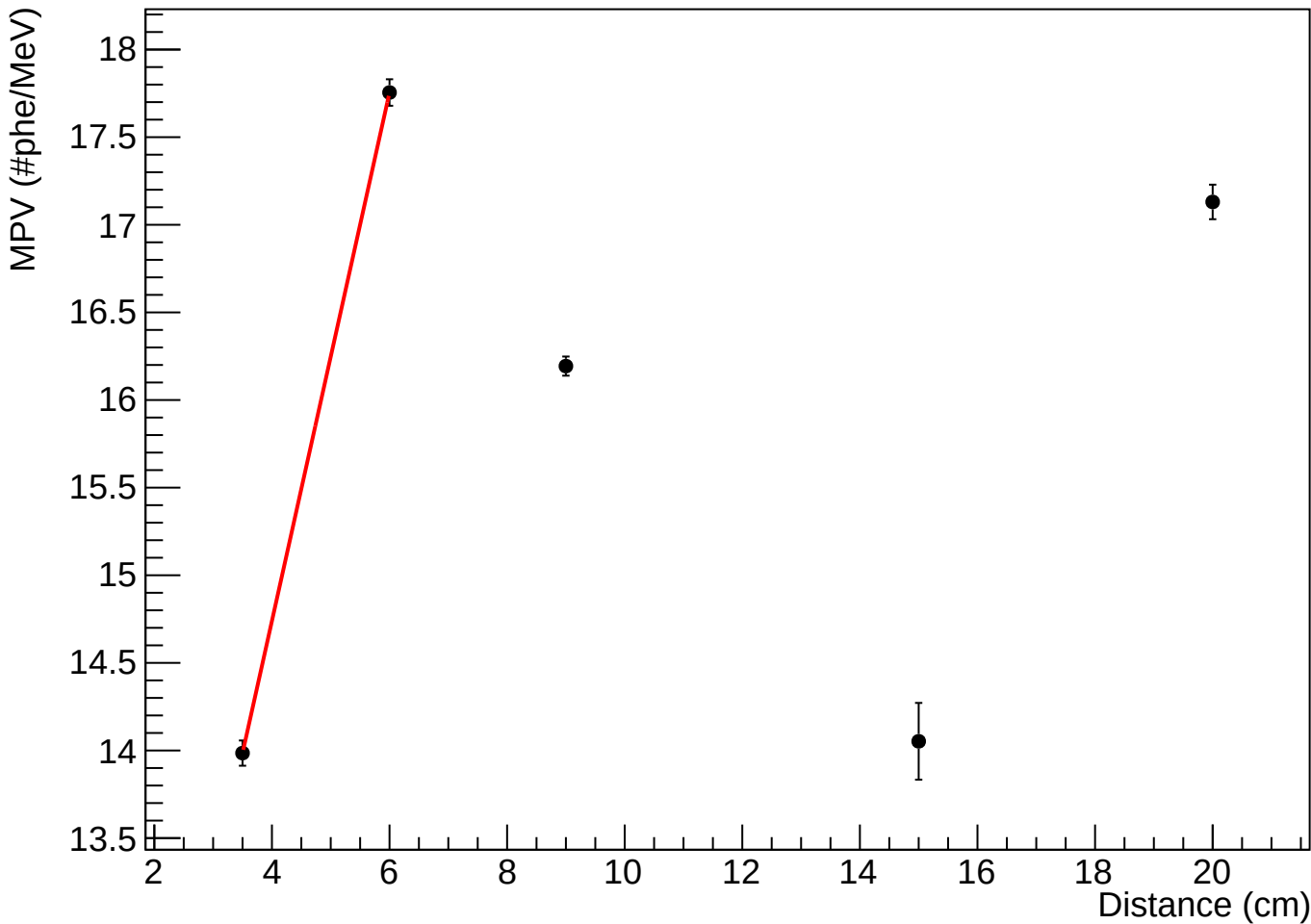
MPV vs Distance from SiPM (using charge)
