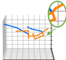
3DHP
