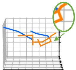
Ground Truth
