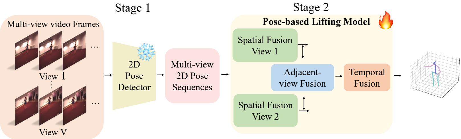
(a) Single-stream multi-view 3D HPE lifting methods
