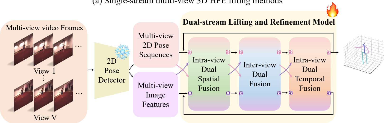
(b) Our dual-stream multi-view 3D HPE lifting and refinement method
