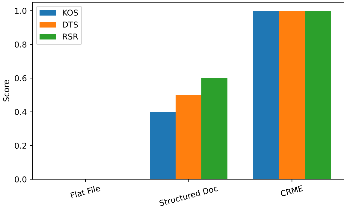
Benchmark Comparison of Research Memory Approaches
