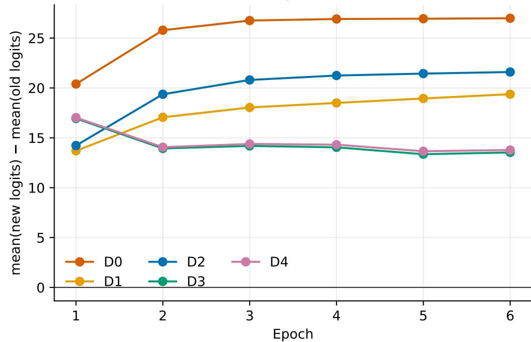
Old/new logit scale drift
