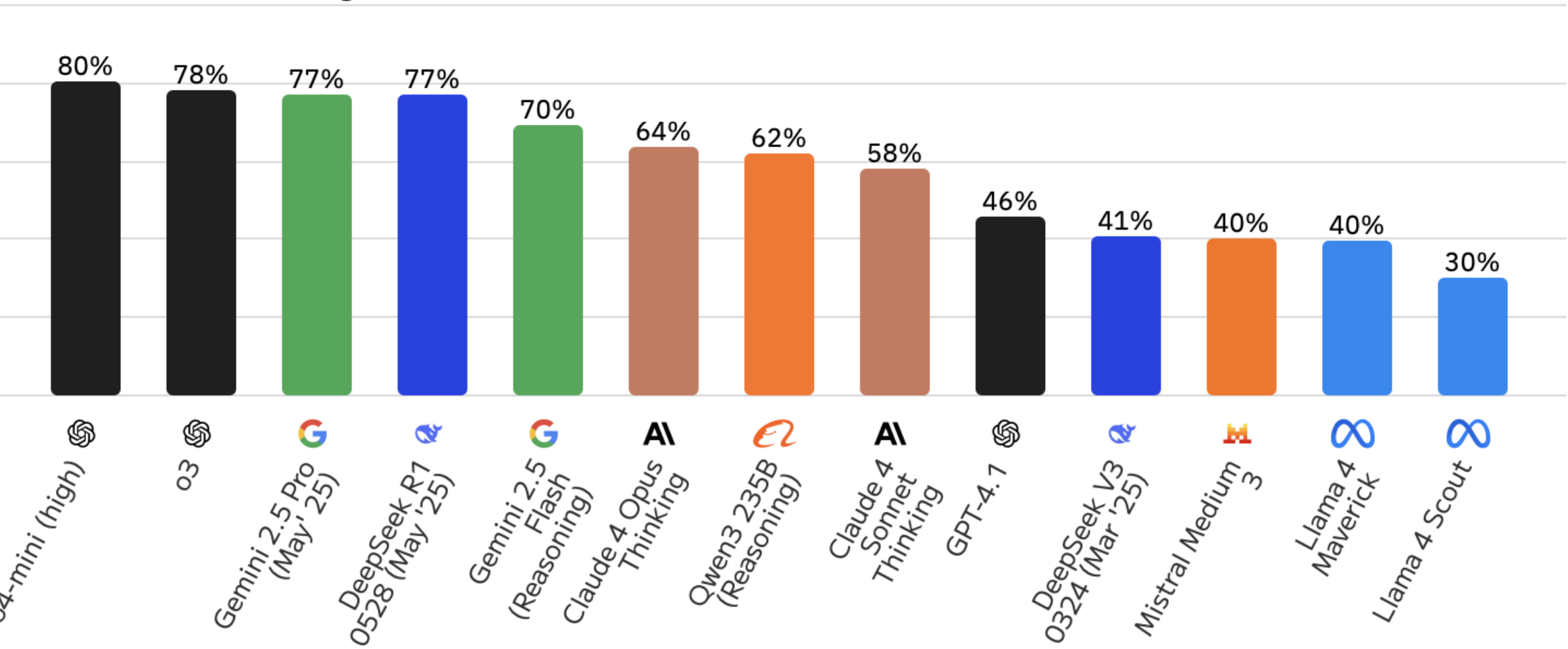
LiveCodeBench (Coding)
