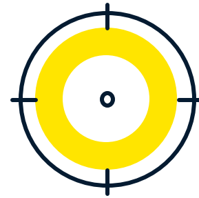
Mistral medium
