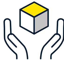
Mistral small
