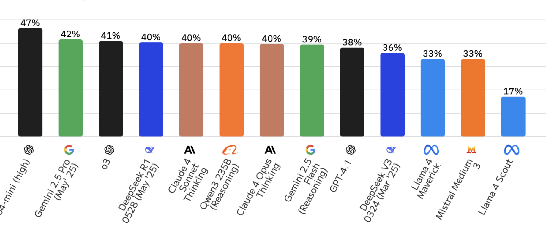
SciCode (Coding)
