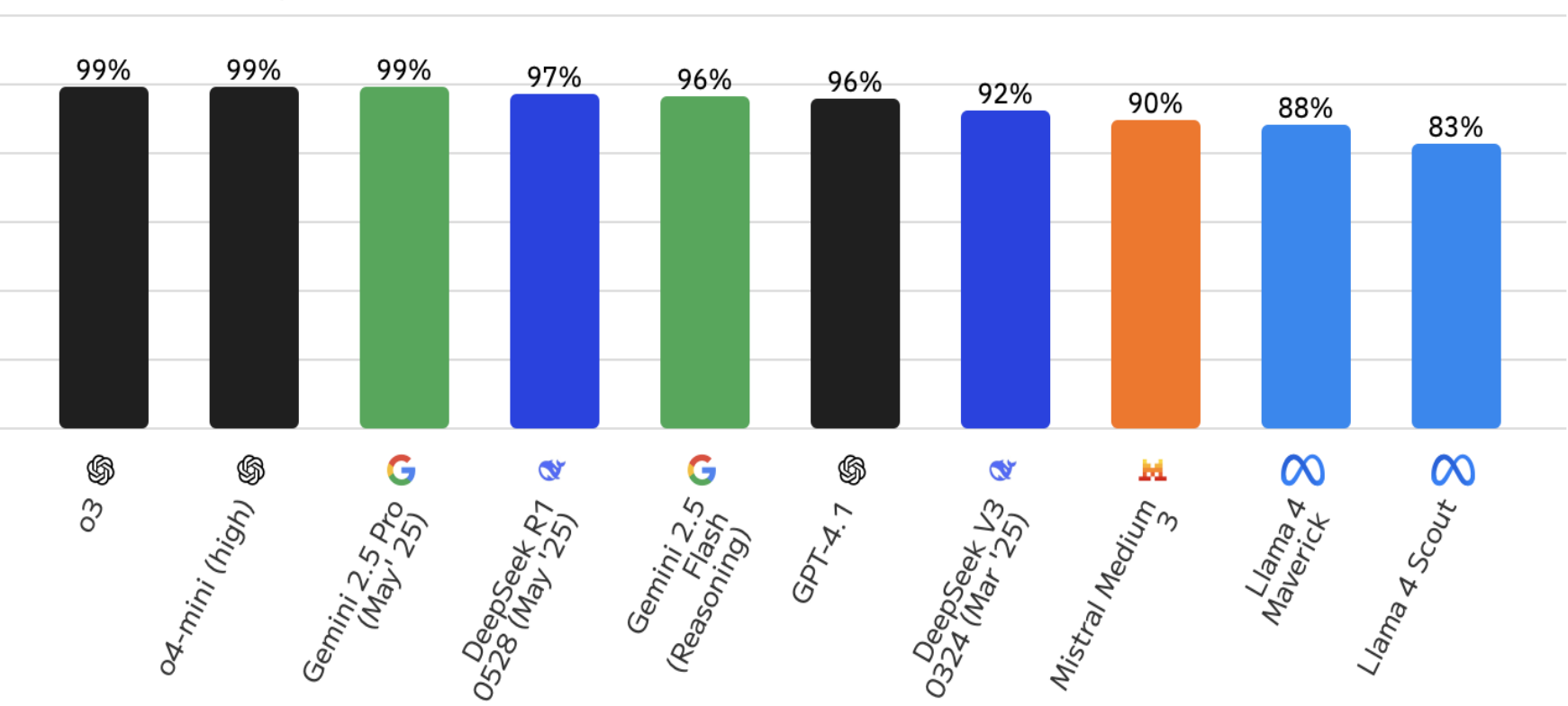
HumanEval (Coding)
