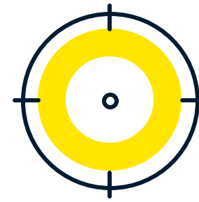
Qwen 2.5 VL
