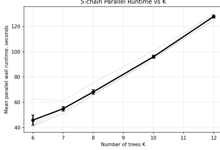
Figure 13: Runtime behavior of HierBOSSS across different values of K for the oxide perovskite dataset. The wall-clock runtime for 5 parallel chains across 5 splits has been reported, with the mean trend in black and split-level variability shown in gray.
