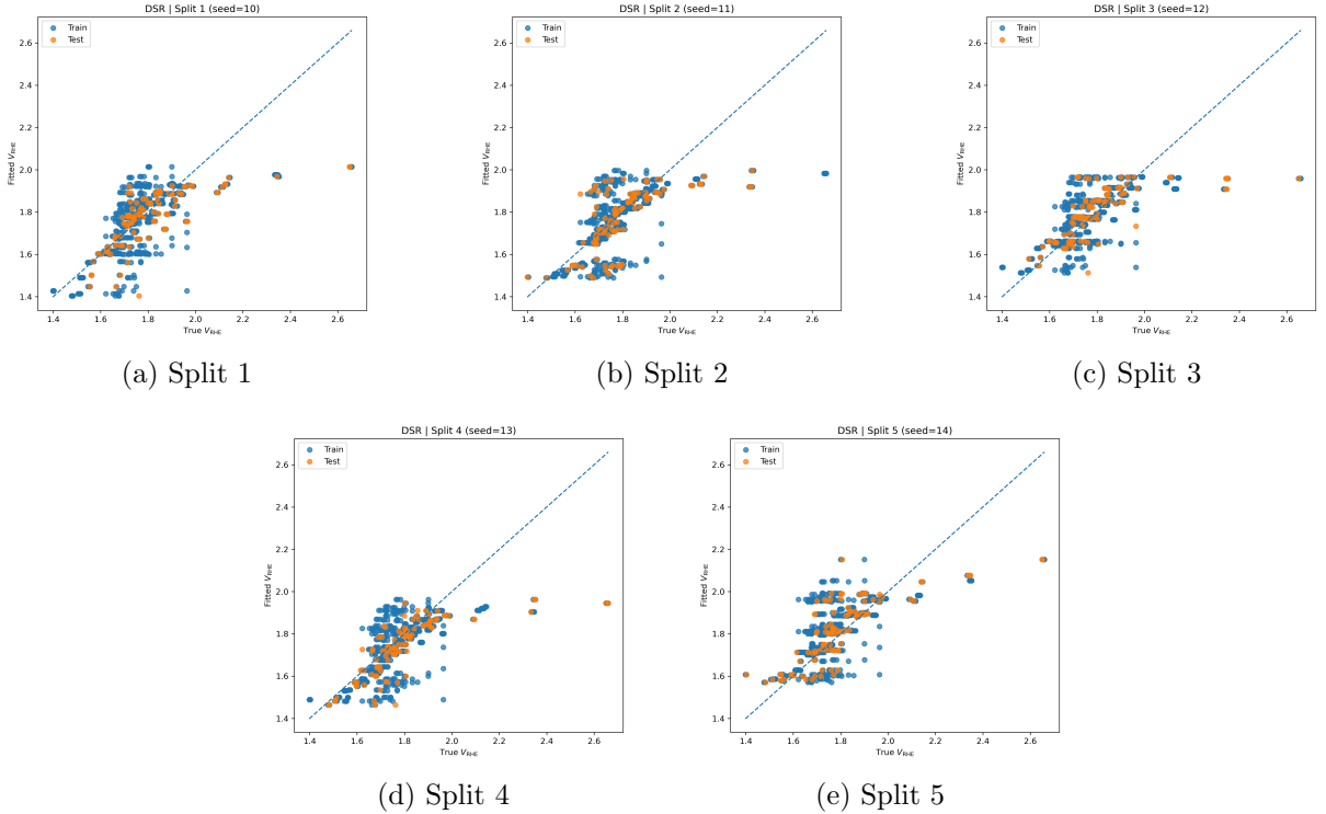
Figure 2: True versus fitted V_{RHE} values obtained by DSR across 5 independent 90/10 train/test splits of the oxide perovskite dataset.
