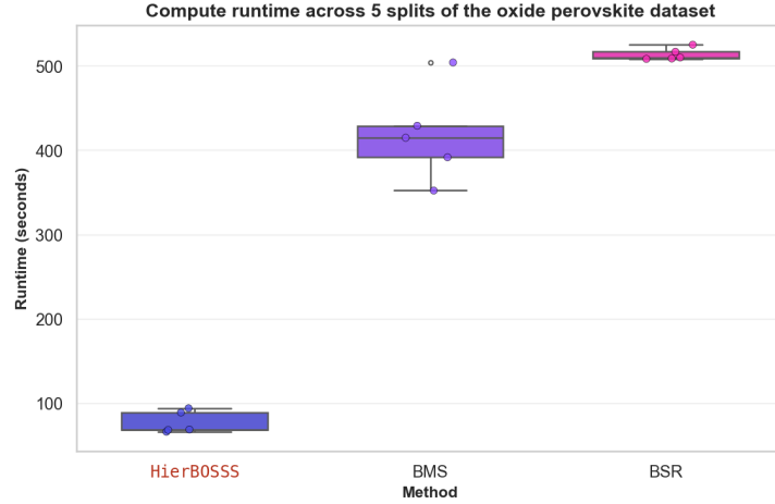
Figure 17: Compute runtimes of HierBOSSS, BMS (5 parallel MCMC chains), and BSR (5 restarts) across 5 splits of the oxide perovskite dataset. Implementation details of HierBOSSS and the Bayesian competitors follow from Section B.1, B.8, and B.9.
