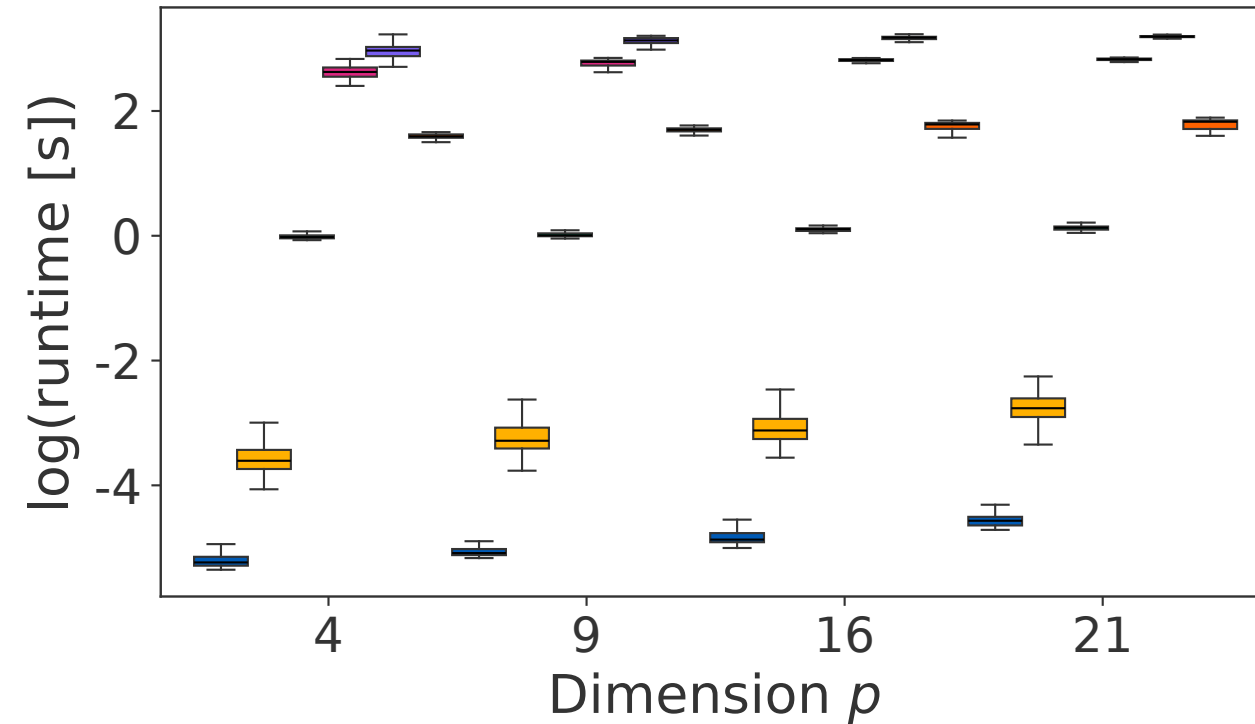
Student- t : varying dimension
