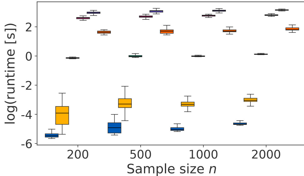
Student- t : varying sample size
