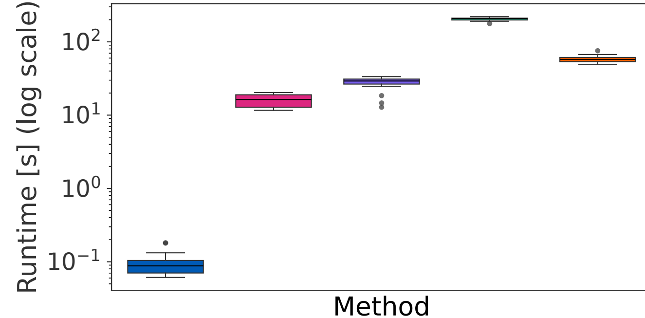
Bayesian quantile regression ( n = 10^4 )
