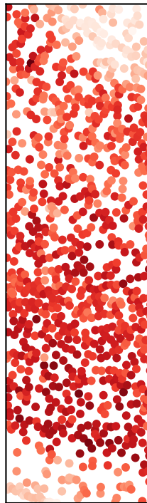
DADVI
