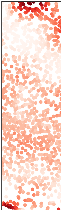
ADVI (MF)
