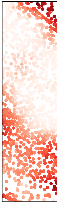
ADVI (MF)
