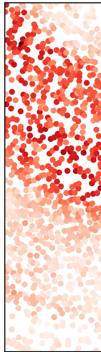
DADVI
