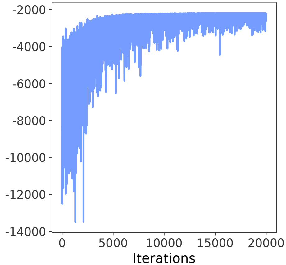
ADVI (MF)
