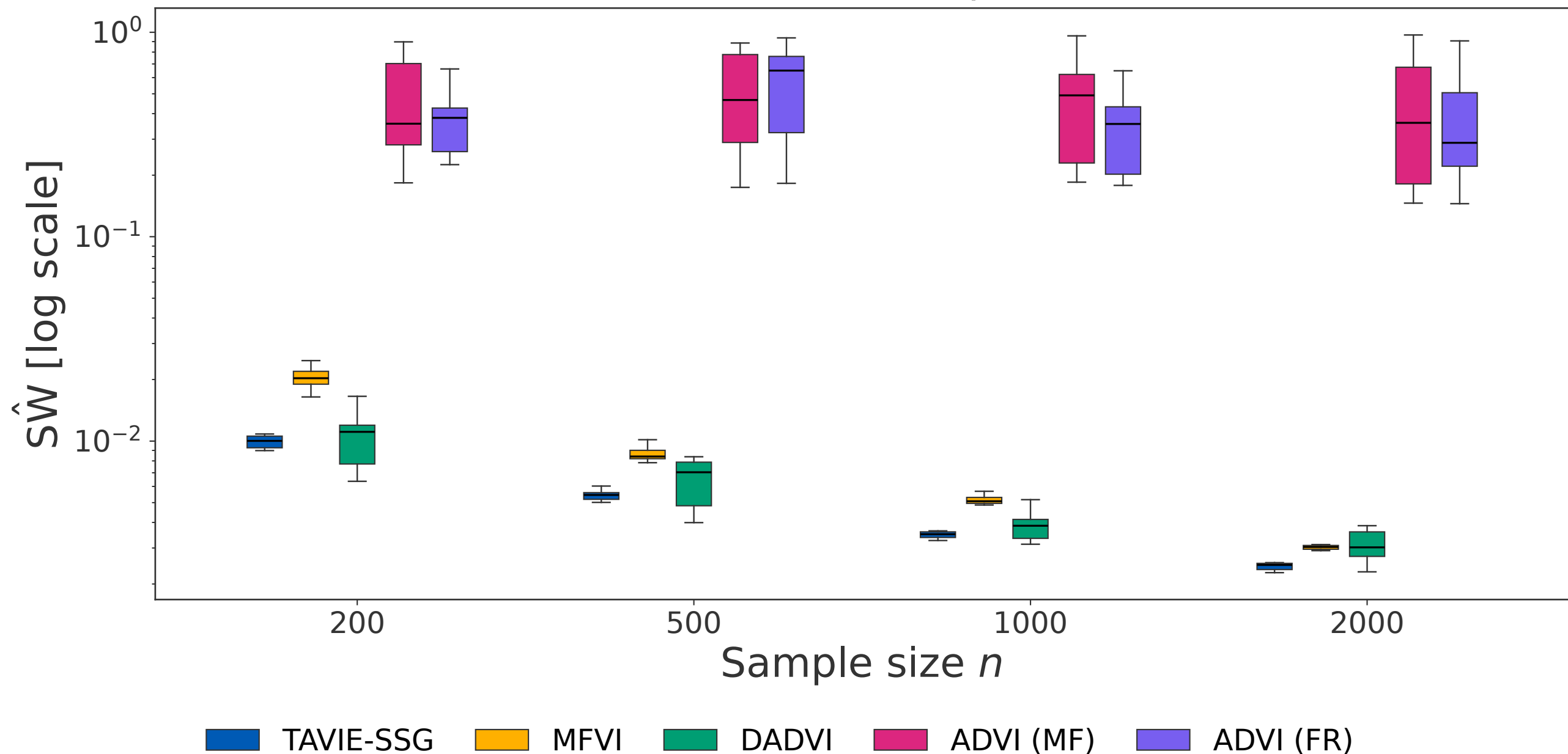
Sliced Wasserstein distance between true and variational posteriors
